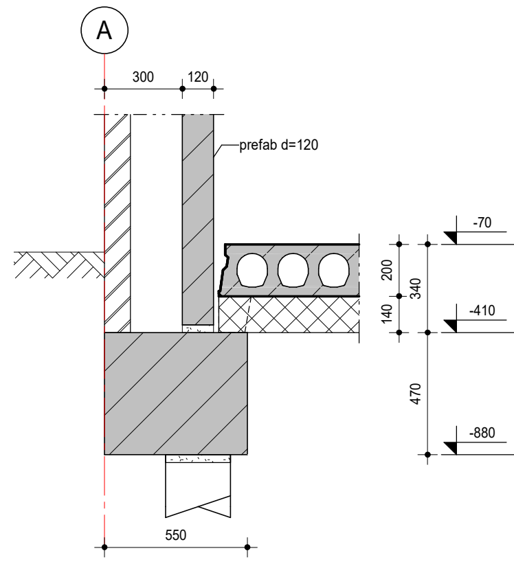
detail 0.03
