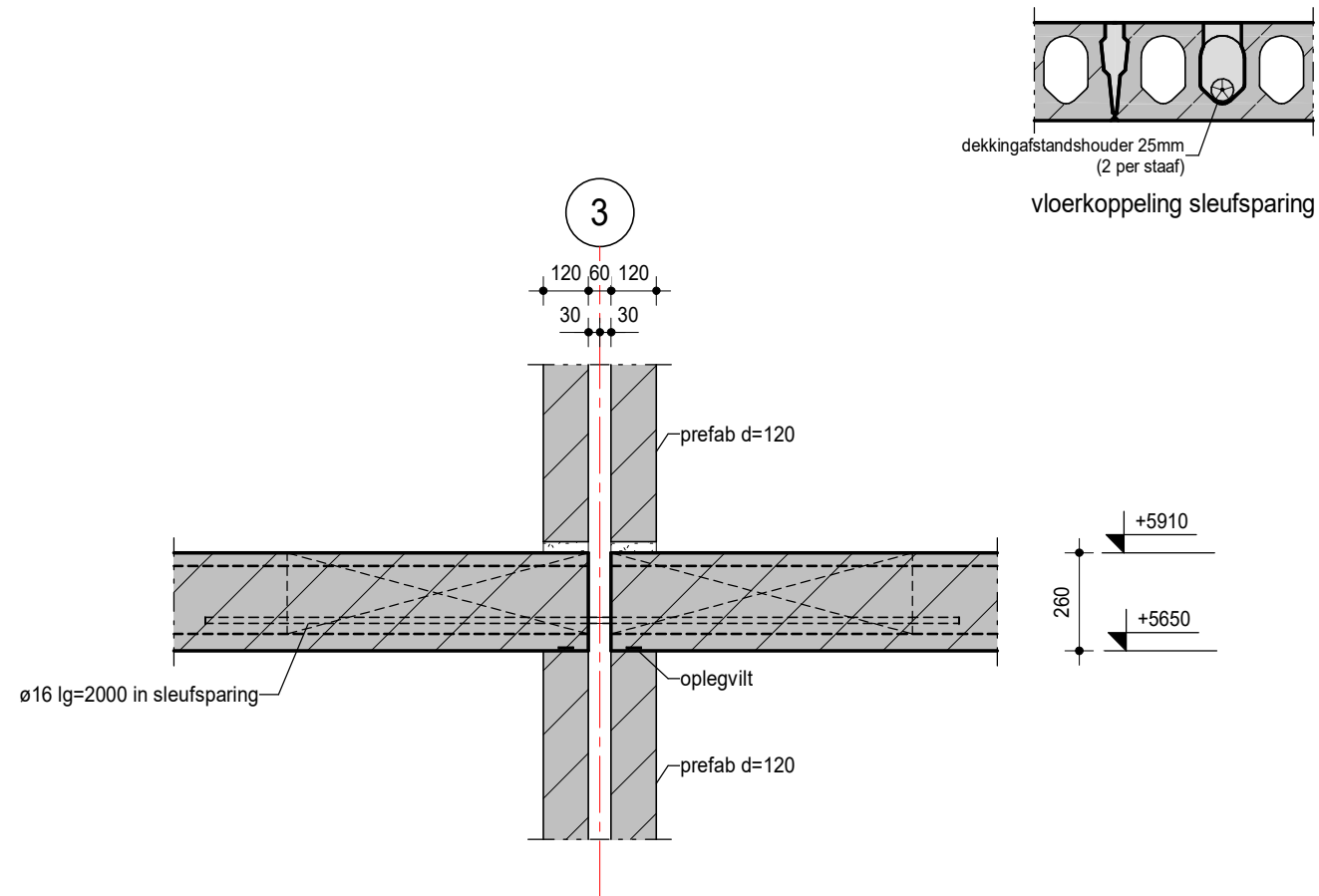
detail 2.02
