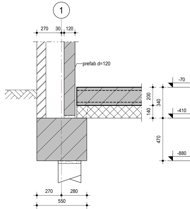
detail 0.01
