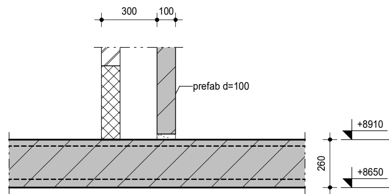
detail 3.02
