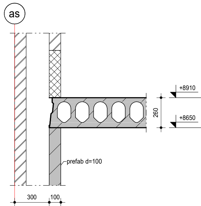
detail 3.06
