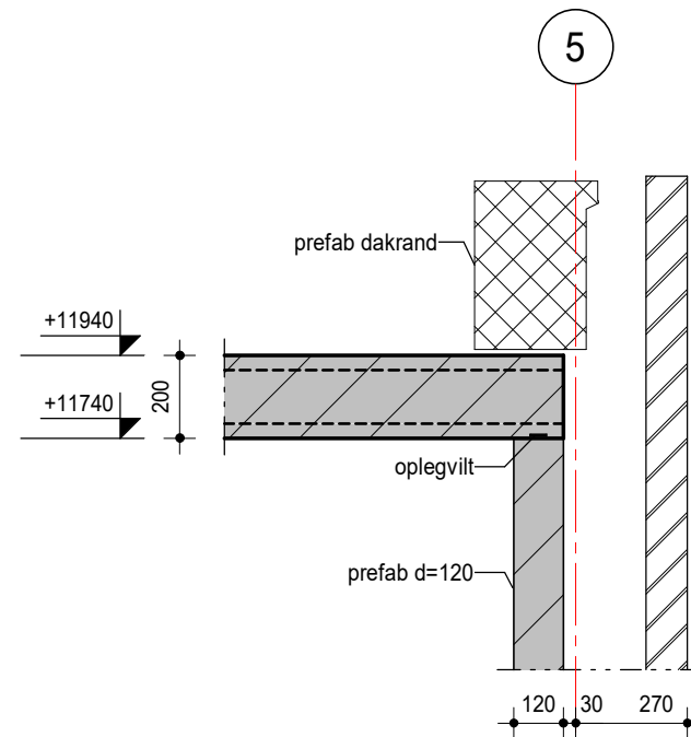
detail 4.03
