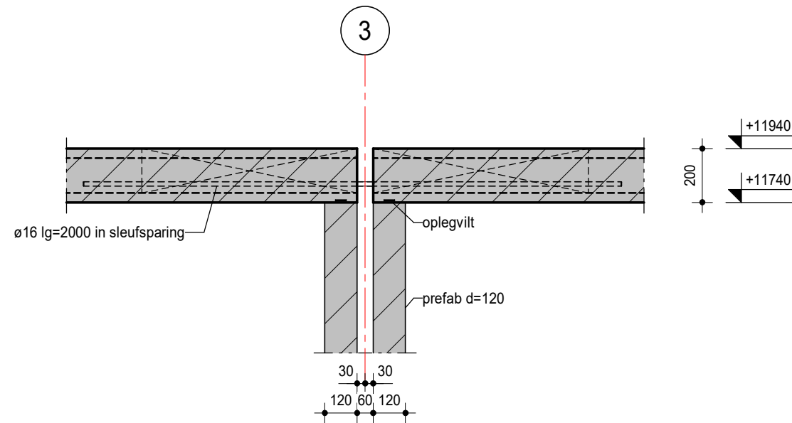
detail 4.02
