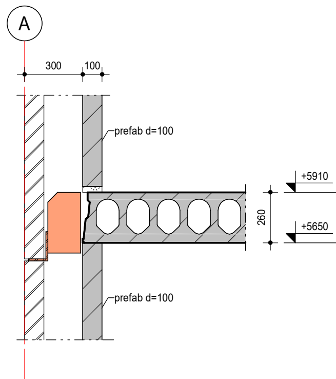
detail 2.03
