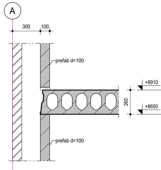
detail 3.07
