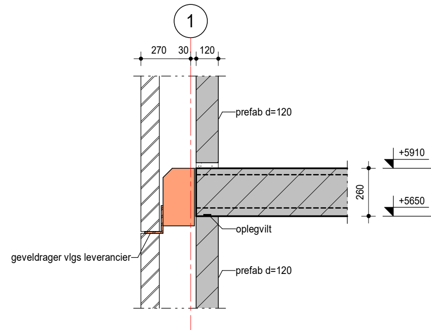
detail 2.01
