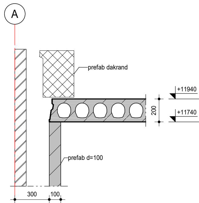
detail 4.04
