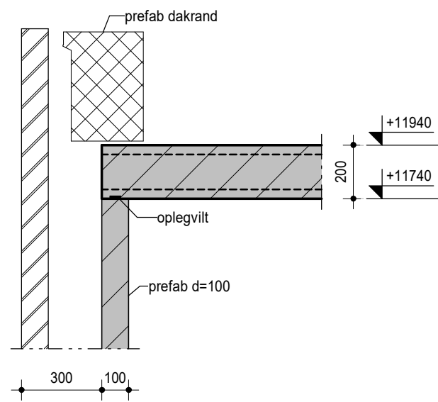
detail 4.01
