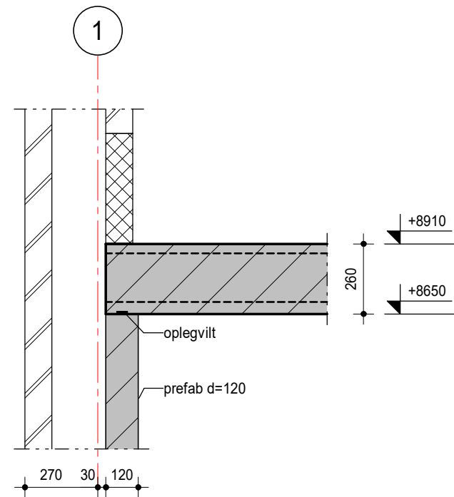
detail 3.01
