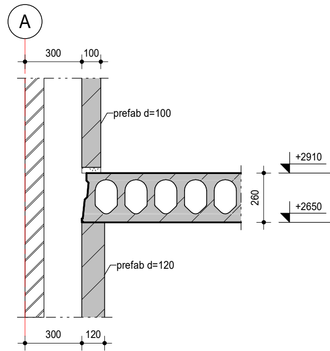
detail 1.04
