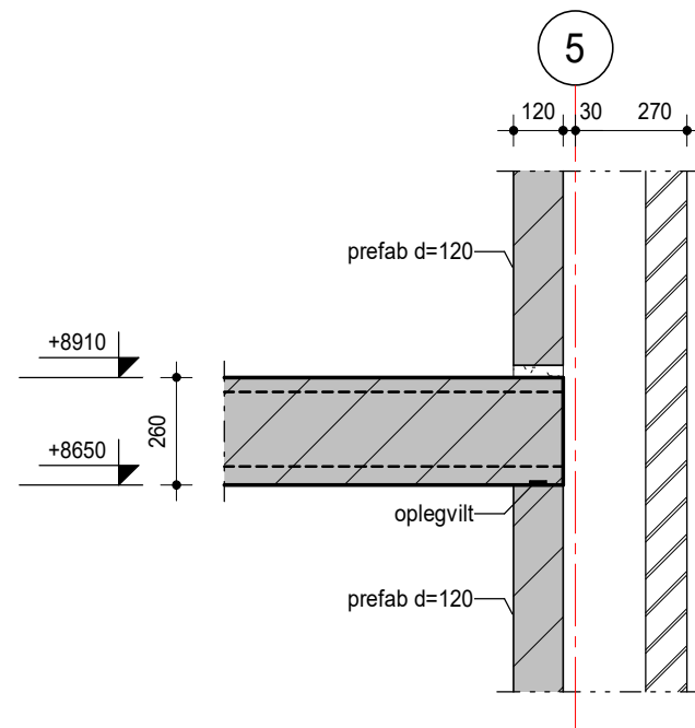
detail 3.05
