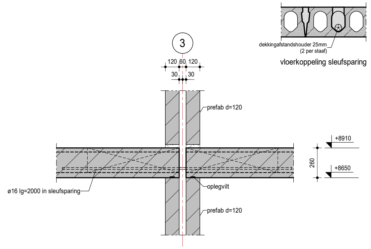
detail 3.04
