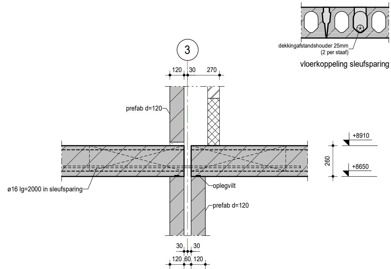
detail 3.03
