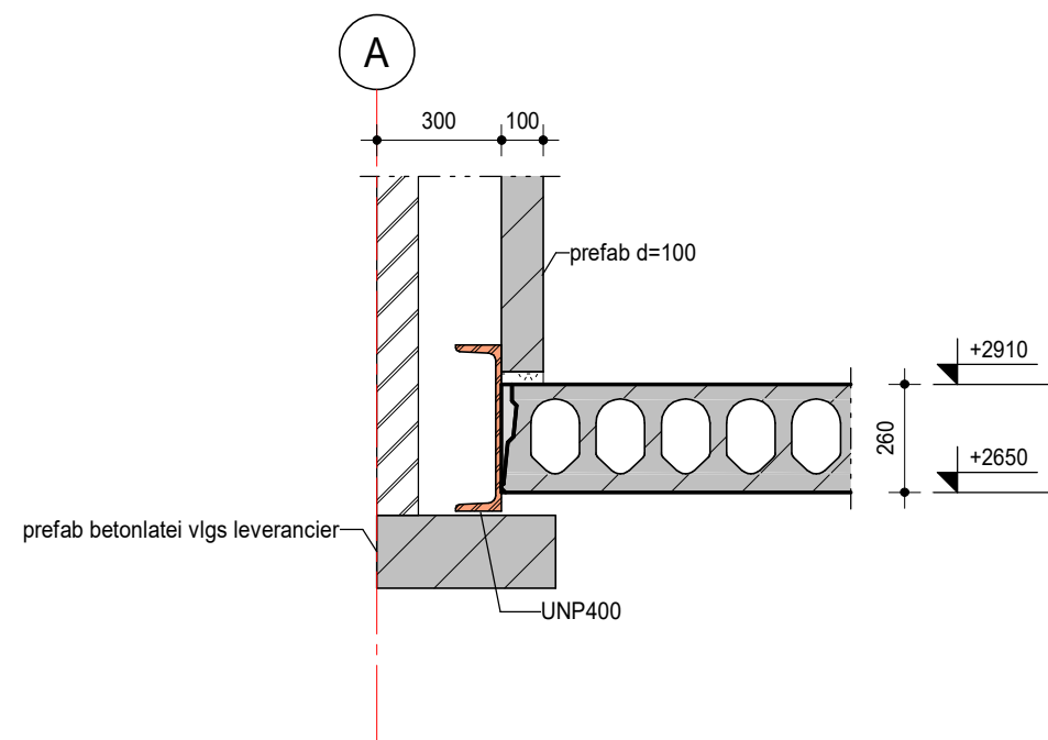
detail 1.05
