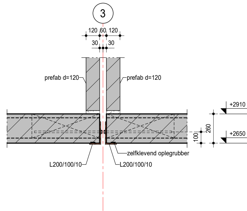
detail 1.03
